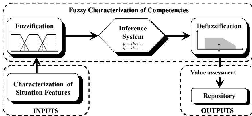
Figure 10: Fuzzy system of competency characterisation
