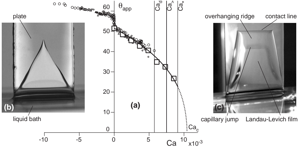
FIGURE 3. (a) Symbols ( \square ): apparent contact angle \theta_{\text{app}} , defined from Eq (4.2) as a function of capillary number for PDMS on fluorinated glass or silicon. Symbols ( \circ , \diamond , \triangle ): data from Rio et al. 2005 obtained for drops sliding on an inclined plane. Vertical lines indicate threshold capillary numbers Ca_d for the drop experiment, Ca_> "corner" dewetting flow on vertical plate (see text), Ca^* for the entrainment transition in the plate geometry. The solid line is the result of the hydrodynamic theory for (\theta_a + \theta_r)/2 , shifted down by 2.8^\circ . It is mostly used as a guide eye but shows that the prediction is within the experimental error on the absolute position of the contact line. (b) Triangular liquid film observed when the dewetting lines originating at the wafer edges meet. (c) Overall shape of the liquid film well above the entrainment transition. Most of the analysis pertains to the horizontal contact line at the top of the film.
