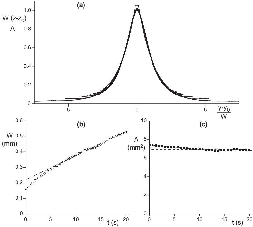
FIGURE 11. (a) Rescaled contact line profiles (from figure 10a) showing the self-similar behavior. (b) Time evolution of the width derived from the fit. (c) Time evolution of the area A under each curve.
