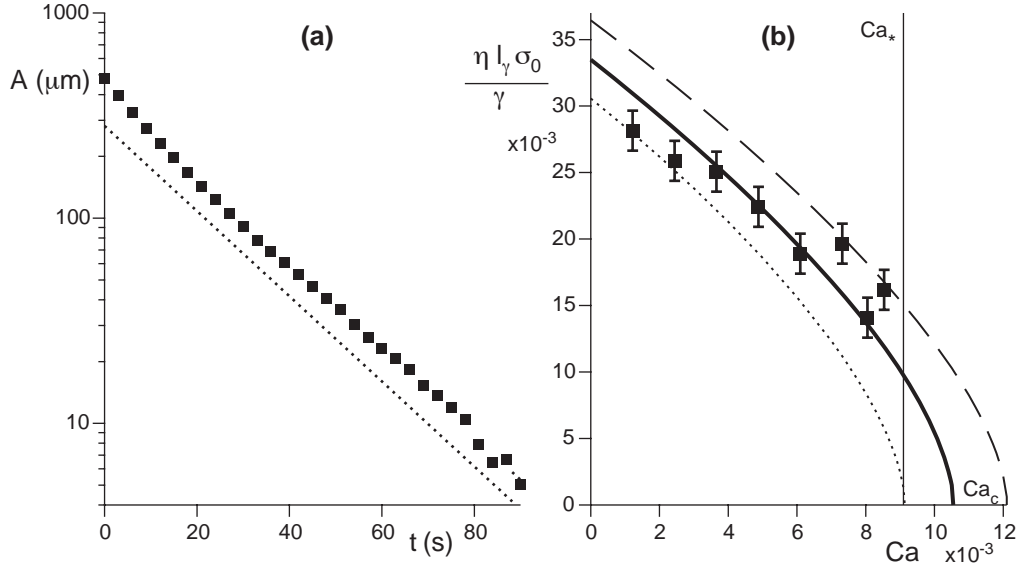
FIGURE 8. (a) Amplitude of contact line perturbation as a function of time for the "zero" mode \lambda \rightarrow \infty . (b) Dimensionless relaxation rate for the zero mode as a function of capillary number. The data have been obtained with the same plate. The error bars indicate the typical variation from one experiment to the other. The lines are the prediction of the multiscale hydrodynamic model for \theta_{cl} = \theta_r (dotted line), (\theta_r + \theta_a)/2 (solid line), \theta_a (dashed line).
