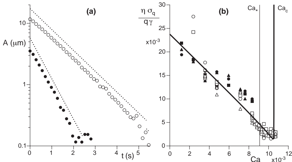
FIGURE 7. (a) Amplitude of contact line deformation as a function of time for periodic perturbations. Open circles \lambda = 400 \mu\text{m} , filled circles \lambda = 200 \mu\text{m} . The dotted lines are exponentials. (b) Dimensionless relaxation rate as a function of capillary number at different wavelengths (defects with 600 \mu\text{m} spacing: ( \circ ) \lambda = 600 \mu , ( \square ) \lambda = 300 \mu , ( \triangle ) \lambda = 200 \mu ; defects with 400 \mu\text{m} spacing: ( \bullet ) \lambda = 400 \mu , ( \blacksquare ) \lambda = 200 \mu , ( \blacktriangle ) \lambda = 133 \mu ). The solid line is the prediction of the multiscale hydrodynamic model with \theta_{cl} = (\theta_a + \theta_r)/2 .
