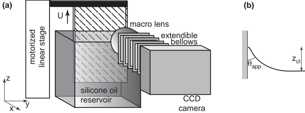
FIGURE 1. Experimental set-up. (a) A vertical plate is withdrawn at velocity U_p from a bath of liquid that does not wet spontaneously on it. (b) Definition of meniscus rise z_{cl} and the apparent contact angle \theta_{app} .
