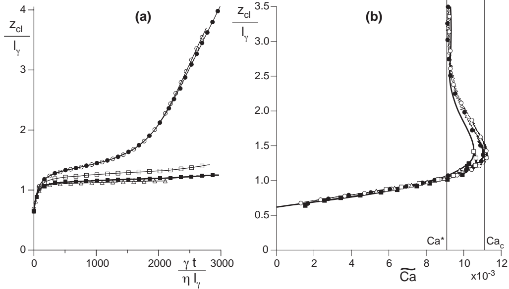
FIGURE 4. (a) Meniscus height z_{cl} rescaled par the capillary length as a function of time, rescaled by the capillary time for Ca = 9.7 \times 10^{-3} ( \Delta ), Ca = 10.2 \times 10^{-3} ( \blacksquare ), Ca = 10.7 \times 10^{-3} ( \square ), Ca = 11.2 \times 10^{-3} ( \bullet ) and Ca = 11.5 \times 10^{-3} ( \circ ). (b) Same data plotted as z_{cl}(t) as a function of the contact line relative capillary number \widetilde{Ca} = \eta(U_p - \dot{z}_{cl}(t))/\gamma . Solid line: Steady solutions of the multi-scale hydrodynamic model.
