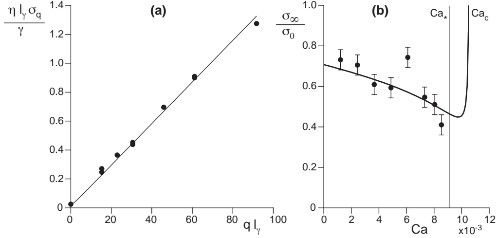
FIGURE 9. (a) Normalized relaxation rate as a function of the wavenumber rescaled by the capillary length. (b) Ratio of the relaxation rate of large wavenumber modes to zero mode rescaled by q l_\gamma , i.e. \sigma_\infty/\sigma_0 . Each point corresponds to an average over several measurements. The error bars indicate the variance around the average. The hydrodynamic theory is presented by a solid line ( \theta_{cl} = (\theta_a + \theta_r)/2 ).
