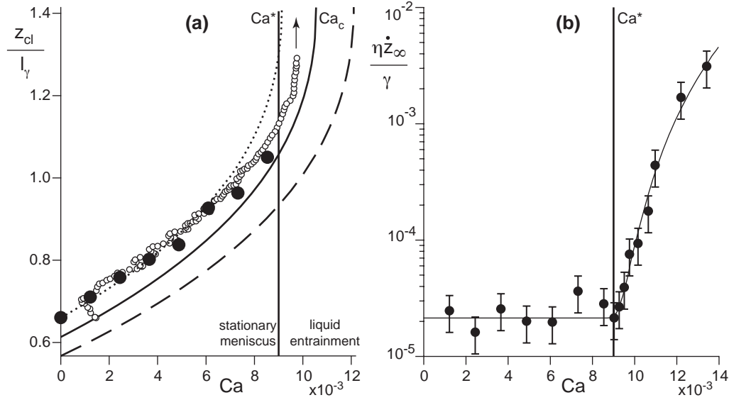
FIGURE 2. (a) Meniscus rise z_{cl} normalized by capillary length l_\gamma as a function of the plate capillary number Ca . Symbols (●): steady solutions, determined experimentally as a function of Ca . Symbols (○): rescaled meniscus rise z_{cl}(t) function of the contact line relative capillary number \widetilde{Ca}(t) = \eta(U_p - \dot{z}_{cl}(t))/\gamma , for Ca = 9.8 \cdot 10^{-3} (see text). Lines: predictions from hydrodynamics theory, with microscopic contact angle \theta_{cl} = \theta_r (dotted), \theta_{cl} = (\theta_a + \theta_r)/2 (solid), \theta_{cl} = \theta_a (dashed). (b) Rescaled contact line velocity at long time \dot{z}_\infty , as a function of the capillary number Ca . Each point corresponds to an average over several experiments. The error bars indicate the typical variation of the measured quantity from one experiment to the other. The solid line is a phenomenological fit of the form: \eta \dot{z}_\infty / \gamma = c_1 + c_2(Ca - Ca^*)^3 . c_1 is a residual ascending velocity present even below the threshold.
