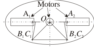
Fig. 11: Placement of the motors and the legs for spherical wrist with parallel actuators
