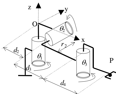
Figure 1 : Orthogonal manipulators under study.
