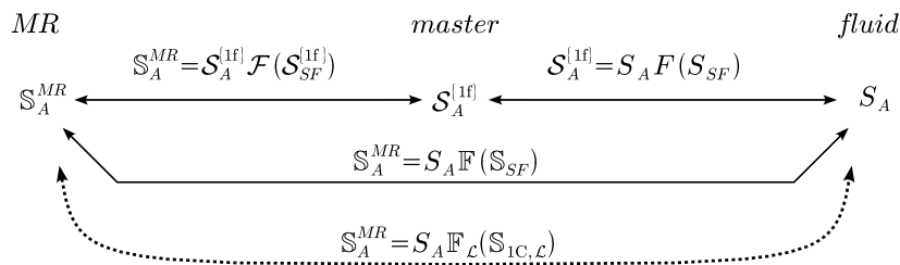
Figure 2: Schematic links between three amplitude characterization \mathbb{S}_A^{\{MR\}} of Eq. (57), \mathcal{S}_A^{\{1f\}} of Eq. (40) and \mathcal{S}_A of Eq. (38), of the theoretical, master and physical singular behaviors, respectively, for a fluid of critical parameters given by Q_c^{\min} = \{(\beta_c)^{-1}, \alpha_c, Y_c, Z_c\} of Eq. (3) and \Lambda_{qe}^* , and which belongs to the one-component fluid subclass.
