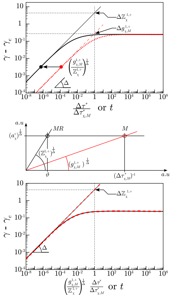
Figure 3: (Color online) Schematic illustrations (for \gamma - \gamma_e and (a_{\chi}^+)^{\frac{1}{\Delta}} ) of the Ising-like preasymptotic equivalence between the dimensionless crossover temperature scale \Delta\tau_{\chi,M}^* needed by the one-parameter crossover model M (dashed red line), and the scale factor \vartheta needed by the massive renormalization (MR) scheme (full black line) [see Eqs. (74), (A2), and (A3), and Table III]; The small difference on the respective \Delta values is neglected.
