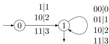
Figure 2: Conversion from base 2 to base 4 (cont.)
