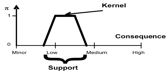
Figure 7: Fuzzy evaluation of the consequence
