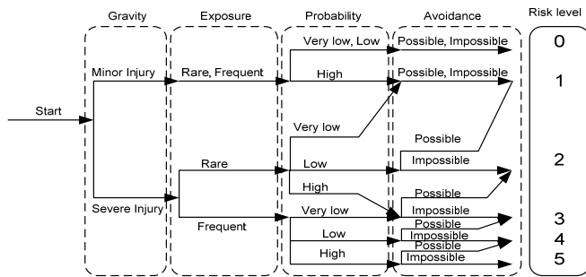
Figure 2: Example of risk graph used by IRSST
