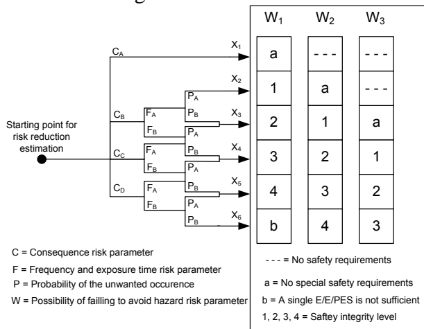
Figure 4: Risk graph in IEC 61508 for SIL allocation
