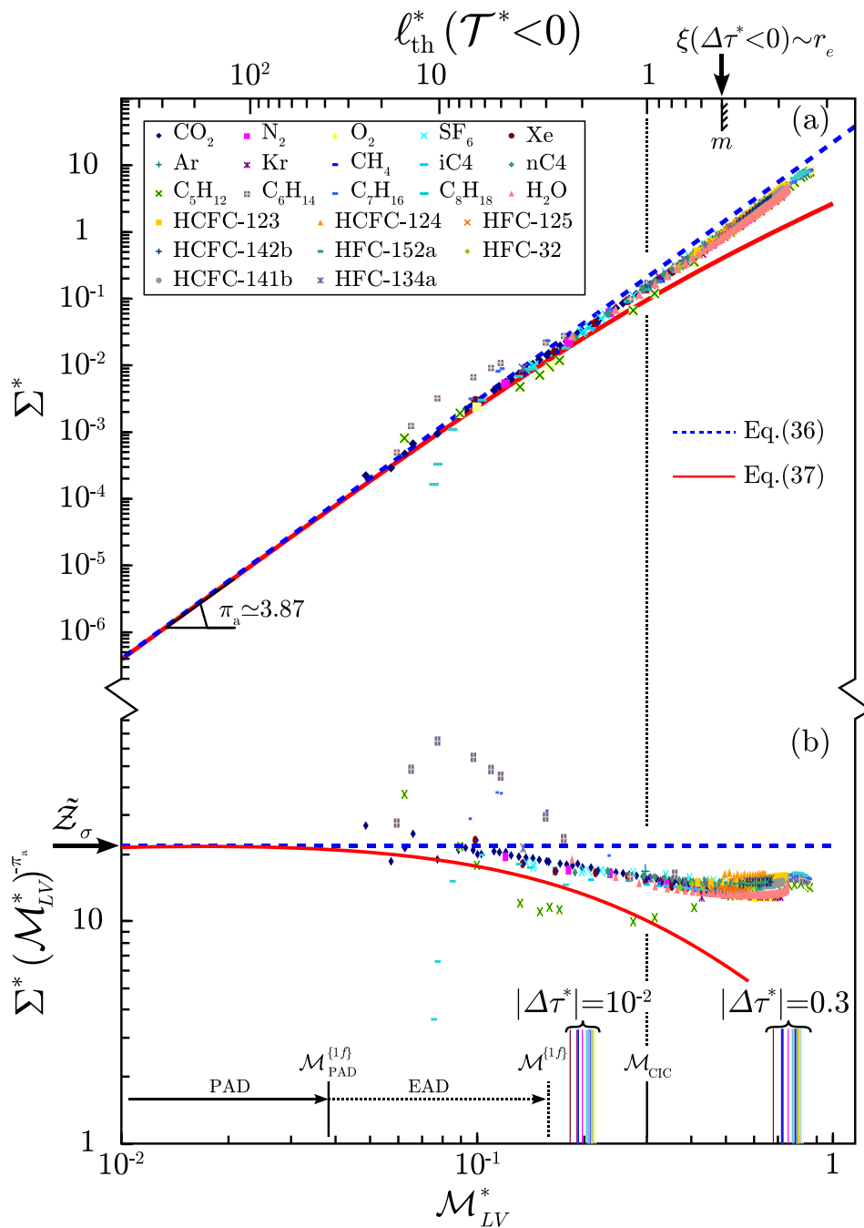
Figure 4: (Colour online) a) Master singular behavior (log-log scale) of the renormalized surface tension \Sigma^* = \sigma^* [Eq. (29)], as a function of the renormalized (symmetrized) order parameter density \mathcal{M}_{LV}^* in the nonhomogeneous domain [see Eq. (28) and text]; b) As in a) for the “confluent” quantity \frac{\Sigma^*}{(\mathcal{M}_{LV}^*)^{\pi_a}} (see text). In a) and b): Dashed blue curve: Eq. (36); full red curve: (37); full arrow with label PAD: \mathcal{M}_{LV}^* < \mathcal{M}_{PAD}^{\{1f\}} extension of the preasymptotic domain; dotted arrow with label EAD: \mathcal{M}_{LV}^* < \mathcal{M}^{\{1f\}} extension of the extended asymptotic domain; The graduation of the upper horizontal axis gives \ell^* (\mathcal{T}^* < 0) calculated from theoretical crossover (see text and Ref. (author?) [51]); arrow sets in lower horizontal axis: |\Delta\tau^*| = 10^{-2} and |\Delta\tau^*| = 0.3 , respectively; Inserted Table gives the fluid color indexation.
