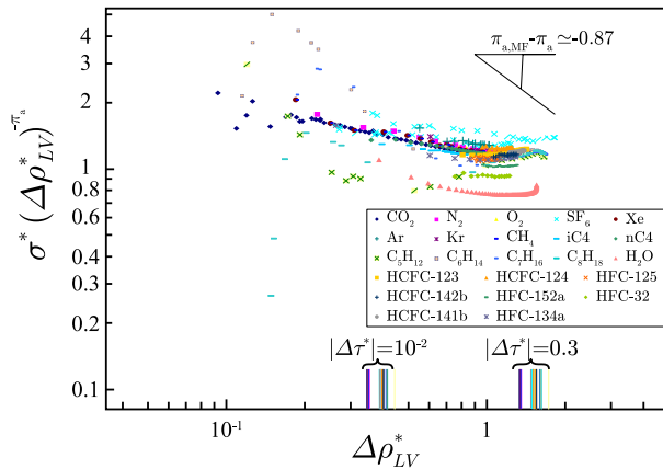
Figure 3: (Color online) Singular behavior (log-log scale) of the dimensionless quantity \frac{\sigma^*}{(\Delta \rho_{LV}^*)^{\pi_a}} as a function of the symmetrized order parameter density \Delta \rho_{LV}^* ; inserted slope: direction difference \pi_{a,MF} - \pi_a = -0.87 from \pi_{a,MF} = 3 (see text); arrow sets in lower horizontal axis: |\Delta \tau^*| = 10^{-2} and |\Delta \tau^*| = 0.3 (see text and caption of 1); Inserted Table gives the fluid colour indexation.
