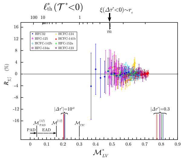
Figure 6: (Color online) lin-lin scale: Residuals (expressed in %) for the experimental master parachor of eight HFCs and HCFCs (see Refs. (author?) [56, 57, 58, 59]), from reference to the master parachor calculated by Eq. (A11).
