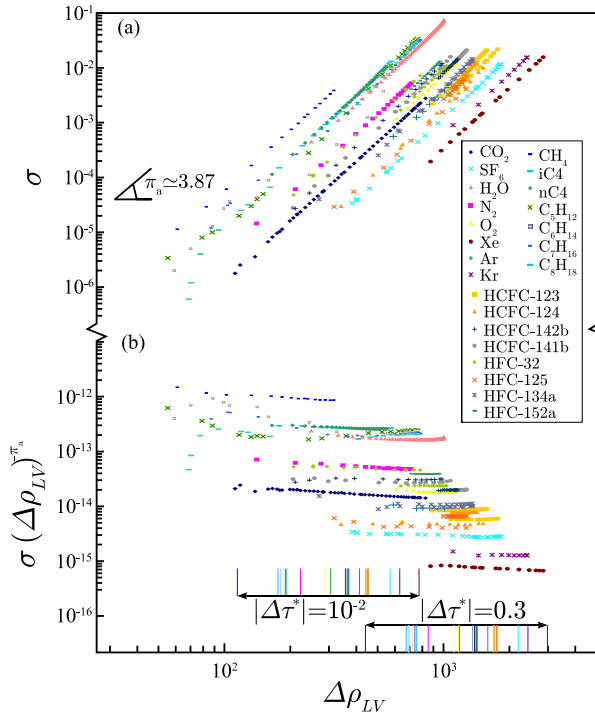
Figure 2: (Color on line) a) Asymptotic singular behavior of \sigma as a function of \Delta\rho_{LV} obtained from Fig. 1 b) As in a) for the confluent quantity \frac{\sigma}{(\Delta\rho_{LV})^{\pi_a}} (see caption of Fig. 1 and text for details and inserted Table for fluid colour indexation).
