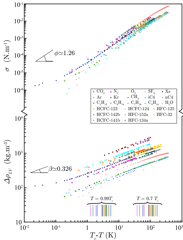
Figure 1: (Color online) a) Singular behavior (log-log scale) of the interfacial tension \sigma (expressed in \text{N}\cdot\text{m}^{-1} ) and b) singular behavior of the symmetrized order parameter density \Delta\rho_{LV} (expressed in \text{kg}\cdot\text{m}^{-3} ), as a function of the temperature distance T_c - T (expressed in K), for one-component fluids (see text, Appendix A and references in Table I). Inserted Table gives colour indexation of each selected fluid. The temperature axis is labelled by vertical arrows which indicate the practical values T = 0.99T_c and T = 0.7T_c , respectively (see text for details).
