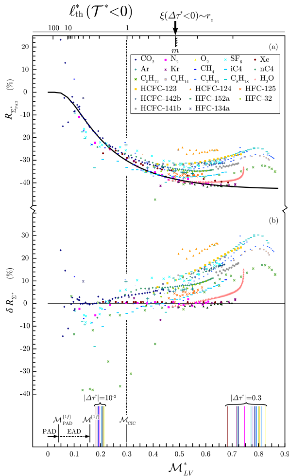
Figure 5: (Color online) lin-lin scale: a) Residuals (expressed in %) for the experimental master parachor from reference to the asymptotical master parachor calculated by Eq. (36), as a function of the master order parameter density; the full black curve corresponds to Eq. (A2) (see text); b) Deviation (expressed in %) of the experimental residuals estimated in part (a), from reference to the full black curve of Eq. (A2).
