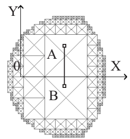
Fig. 7: Workspace and collision-free workspace
