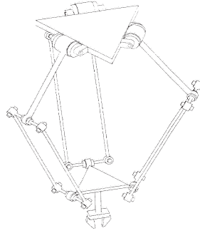
Figure 3: The Delta manipulator
