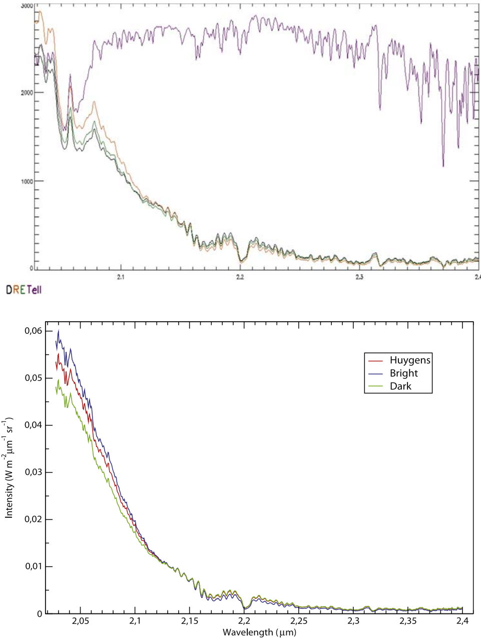
Figure 2. (top) Raw spectra (analog-to-digital unit versus wavelength) of the three regions (E in green, R in gold, D in black), with the spectrum of a standard photometric star (in violet, fitted to the telluric features on the Huygens landing site) to help us correct for the terrestrial atmospheric absorption features (mainly shortward of 2.1 \mu\text{m} and longward of 2.3 \mu\text{m} ). (bottom) Calibrated spectra in \text{W m}^{-2} \mu\text{m}^{-1} \text{sr}^{-1} of the three regions of interest here. We use the data in the methane band, longward of 2.12 \mu\text{m} , to fix the atmospheric parameters. As a second step, with the atmospheric profile fixed, we let the surface albedo be the only variable parameter to fit in the methane window.
