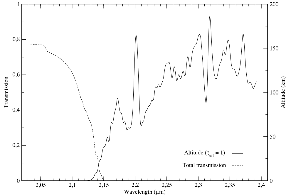
Figure 5. Altitude probed and total transmission (haze + gas) as a function of wavelength. The transmission of 0.8 near the center of the methane window is mainly due to the haze contribution to the total transmission (see text for details).
