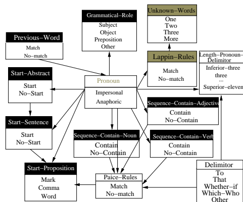
Figure 2: A Bayesian Network for impersonal it classification
