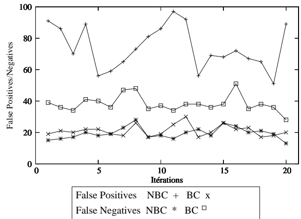
Figure 3: Prediction Results (Accuracy/False Positive Cases/False Negatives Cases)
