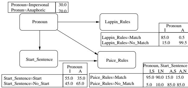
Figure 1: Example of a bayesian classifier modeled by a bayesian network
