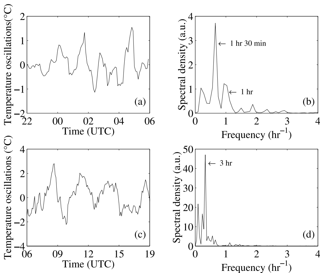
Figure 14. (a) Time series of the temperature oscillations on the night of 25 June at Vallon d'Ol between 2200 and 0600 UTC (b) with its corresponding power spectrum (obtained using a Bayesian spectral estimator). (c and d) Same as Figures 14a and 14b except for the time series between 0600 and 1900 UTC. Adapted from Bastin and Drobinski [2005], with kind permission of Springer Science and Business Media.
