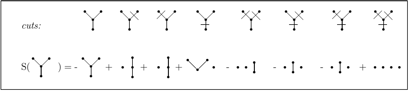
Figure 3: the antipode.
