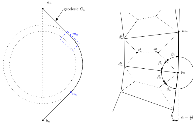
Figure 3: Triangulation T_n and geodesic C_n seen from above: on the left we see the whole surface; the region in the dashed rectangle is depicted on the right
