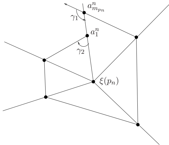
Figure 8: Projection of C_n onto the plane \Pi_{\xi(p_n)}^S (Proposition 4 - case 1)
