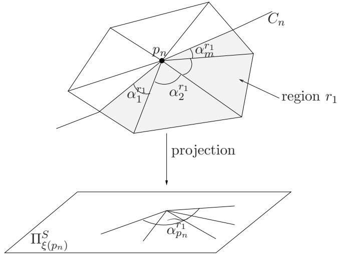
Figure 7: Proof of Proposition 3 - Case 2
