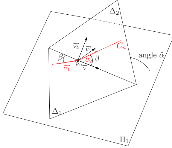
Figure 6: Proof of Proposition 3 - Case 1
