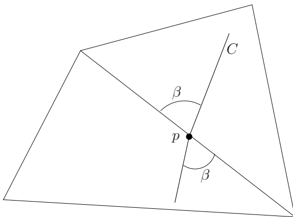
Figure 1: A geodesic C passing through an edge of a 3D triangulation
