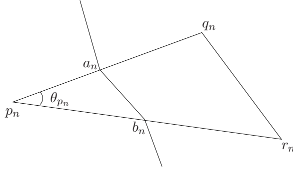
Figure 9: Proof of Proposition 4 - case 2
