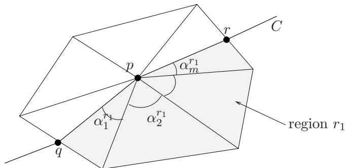
Figure 2: A geodesic C passing through a vertex of a 3D triangulation
