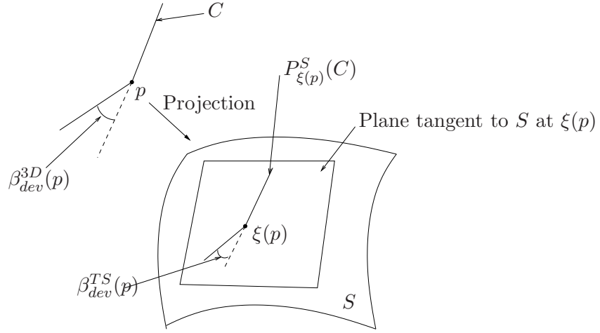
Figure 4: Deviation angle of the curve and of its projection
