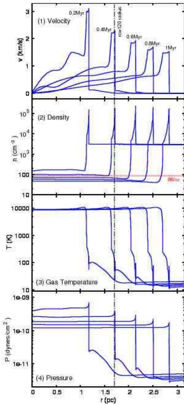
Fig. 14. Snapshots of the gas dynamical evolution at t=0.2, 0.4, 0.6, 0.8, and 1.0 \text{ Myr}
