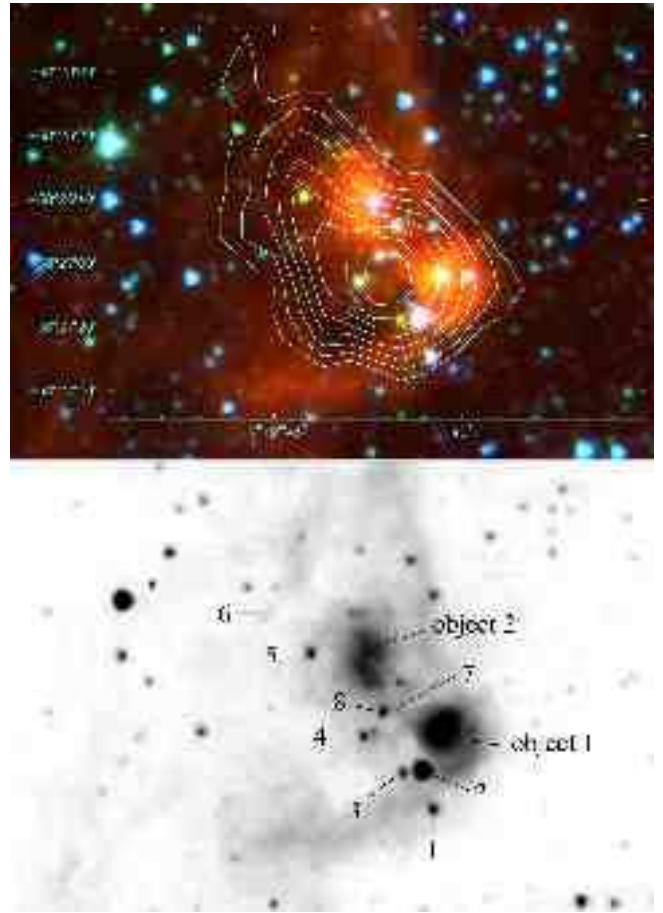
Fig. 8. Top: Same as Fig. 7, but for condensation 4. The sources discussed in the text are identified in the 8\mu\text{m} GLIMPSE image ( bottom )
