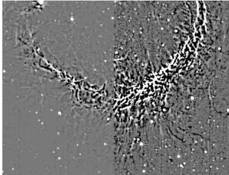
Fig. 13. Unsharp-masked image of the southern part of RCW 120 at 8 \mu\text{m} (see text for details)
