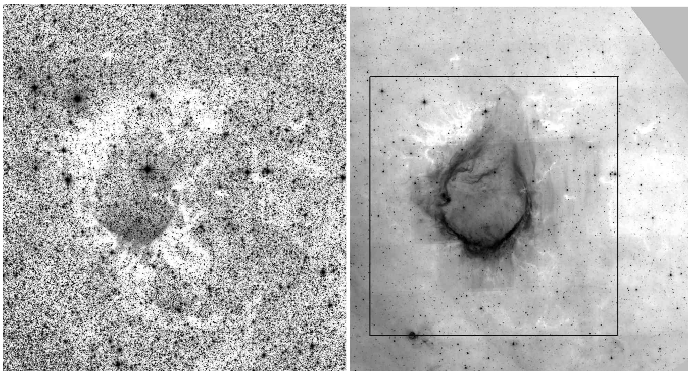
Fig. 3. Dust associated with RCW 120. Left: K_s ( 2.17\ \mu\text{m} ) mosaic image of the RCW 120 region from the 2MASS survey. Zones of high absorption surround the ionized region. Absorption filaments extend far away from the ionization front, revealing a non-homogenous medium. Right: PAH emission at 8\ \mu\text{m} from Spitzer-GLIMPSE. Absorption features are still seen at this wavelength, indicating the presence of dense material. The black box represents the region that has been searched for young stellar objects
