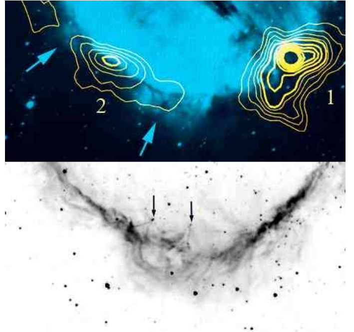
Fig. 12. Instabilities of the ionization front. Top: the ionized gas traced by the H \alpha emission (in blue) leaks between condensations 1 and 2, at the locations shown by the blue arrows. Bottom: structure of the ionization front (GLIMPSE 5.8 \mu\text{m} image). The black arrows point to two YSOs (1H II and 5H II) observed at the vertices of triangular structures possibly created by dynamical instabilities in the ionization front
