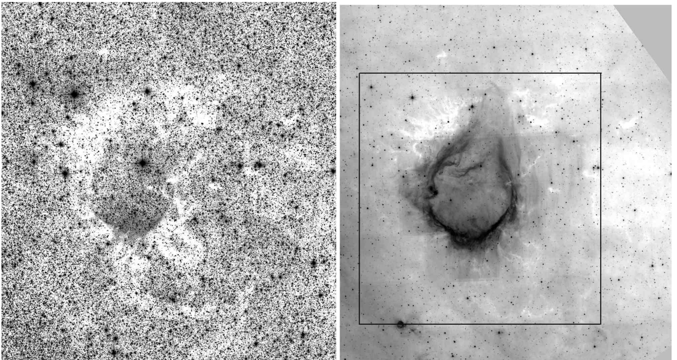
Fig. 3. Dust associated with RCW 120. Left: K_s ( 2.17\ \mu\text{m} ) mosaic image of the RCW 120 region from the 2MASS survey. Zones of high absorption surround the ionized region. Absorption filaments extend far away from the ionization front, revealing a non-homogenous medium. Right: PAH emission at 8\ \mu\text{m} from Spitzer-GLIMPSE. Absorption features are still seen at this wavelength, indicating the presence of dense material. The black box represents the region that has been searched for young stellar objects
