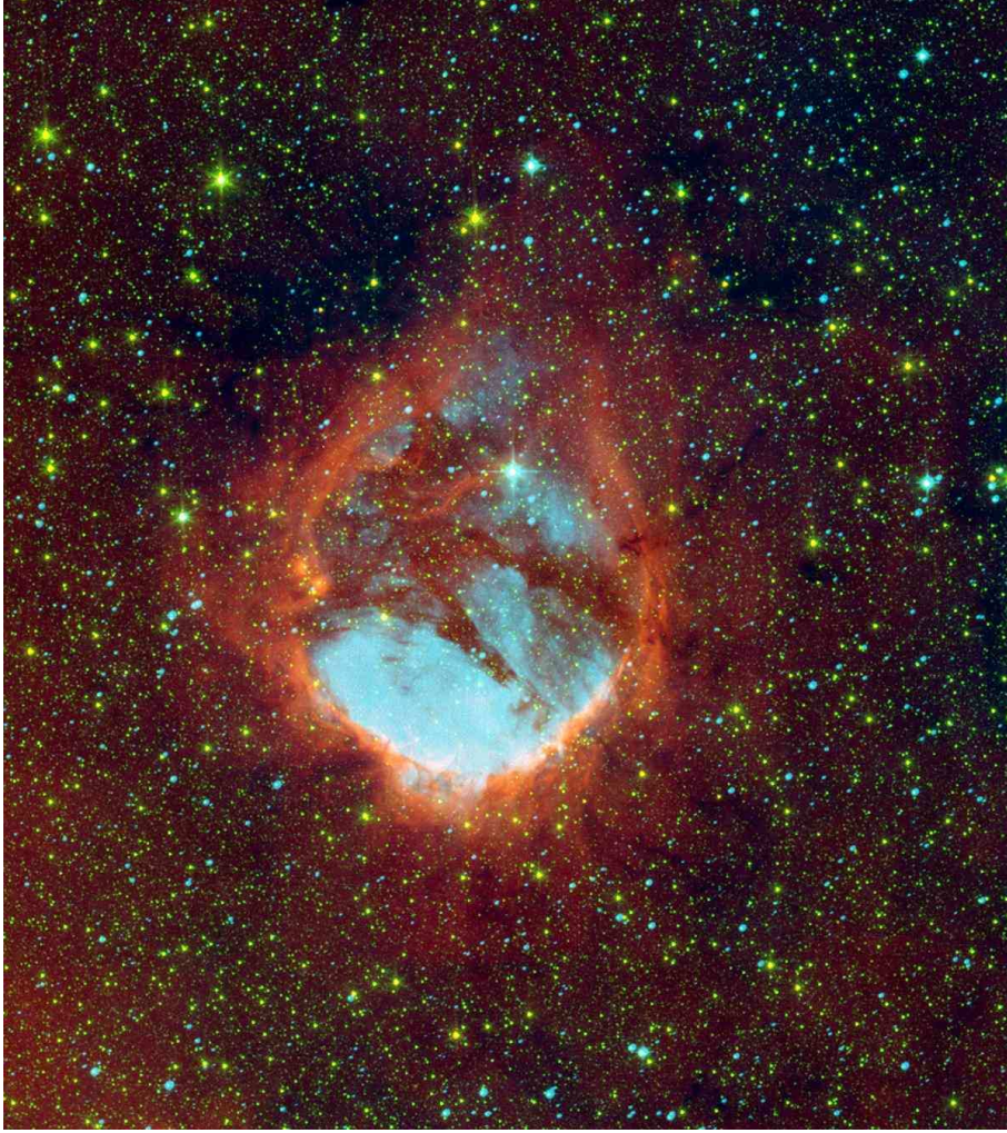
Fig. 2. Spitzer-IRAC 4.5\ \mu\text{m} (green) and 8\ \mu\text{m} (red) images from the GLIMPSE survey superimposed on a SuperCOSMOS \text{H}\alpha image (turquoise) of RCW 120. The 8\ \mu\text{m} emission is dominated by the polycyclic aromatic hydrocarbon (PAH) molecules. Note the presence of a PAH layer, corresponding to the hot photodissociation region that surrounds the ionized region. The field size is 24' (E-W) \times 27' (N-S). North is up and east is left
