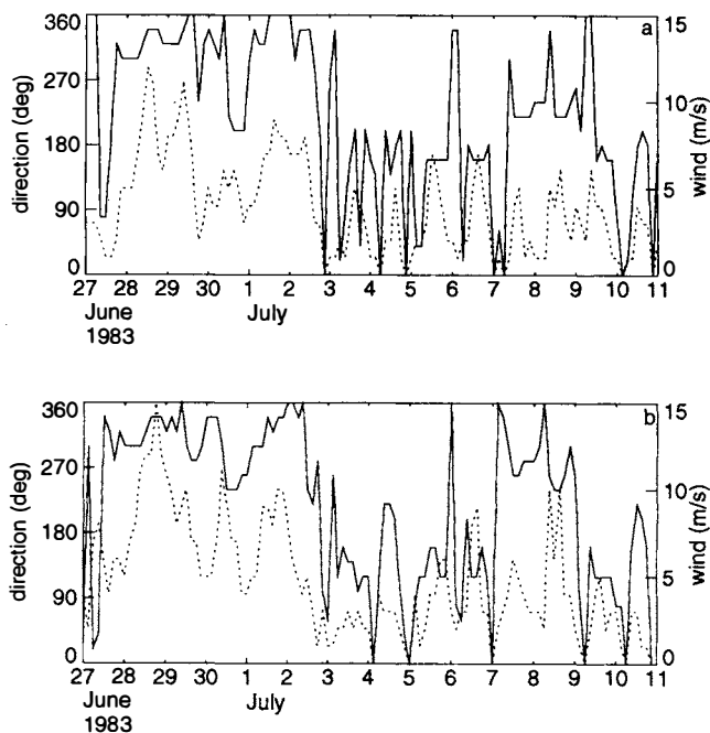
Figure 3. Time series of wind intensities (dashed line) and directions (solid line) respectively recorded at the Tour du Valat (a) and Cap Couronne (b) stations.
