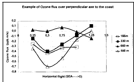
Fig.6. Evolution of ozone fluxes over horizontal runs at various altitudes.
