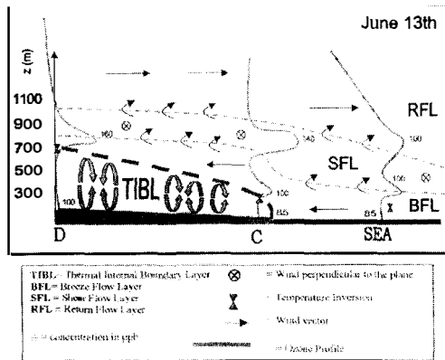
Fig.5. Schematic representation of two dimensional structure of the atmosphere (afternoon 13/06/97) (Cuvelier and al. 1998)
