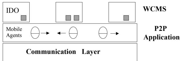
Figure 1. RetroMob Architecture
