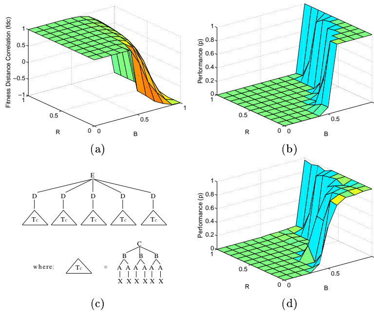
Fig. 1. (a): fdc values for some trap functions obtained by changing the values of the constants B and R . (b): Performance (p) values of SMGP for traps. (d): Performance (p) values of standard GP for traps. (c): Structure of the tree used as optimum in the experiments reported in (a), (b) and (d).
