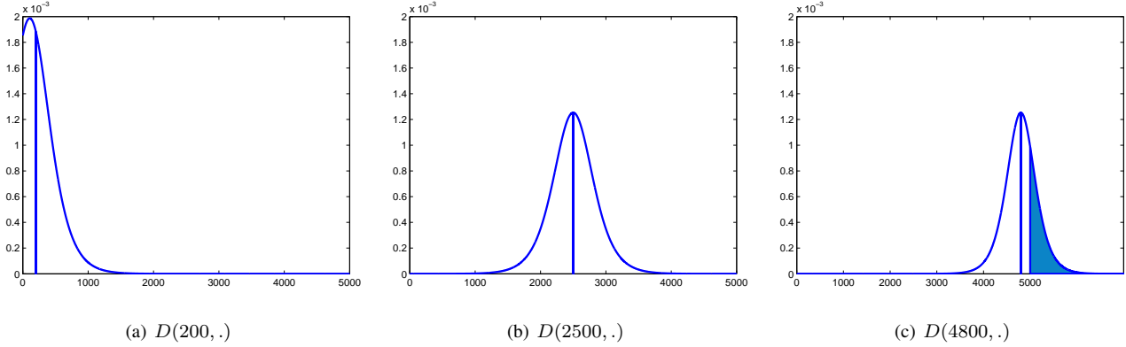
Figure 4. Distribution D(i, \cdot) for three values of i .
