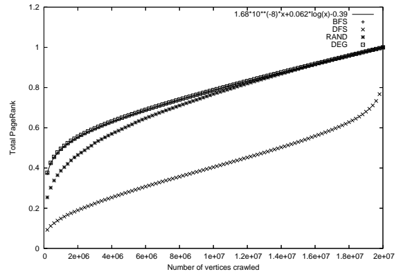
Fig.7 PageRank capture.
