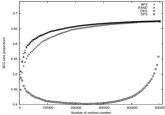
Fig.5 Evolution of the size of the largest SCC (left) and of the OUT pages (right) across time (One seed, up to 500,000 pages in the crawl)
