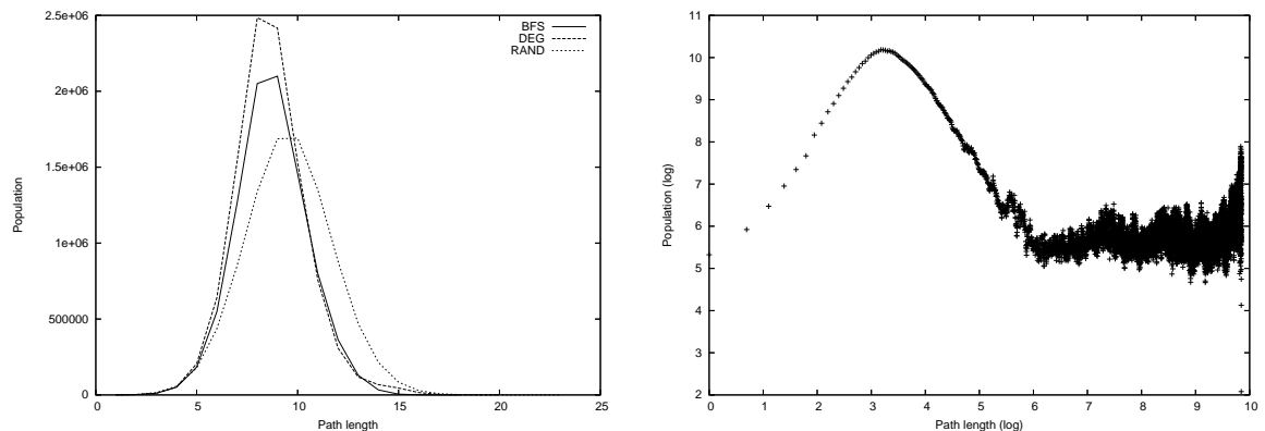
Fig.2 Distribution of path length for BFS and DEG and RAND (left) and DFS (right)
