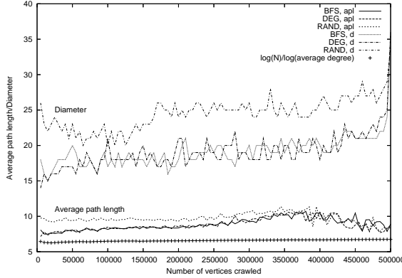
Fig.3 Evolution of diameter and average path length across time for BFS, DEG and RAND
