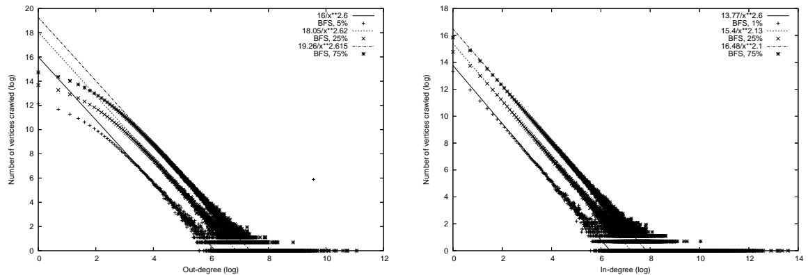
Fig.1 Out-degree distribution (left) and in-degree distribution (right) at three steps of a BFS
