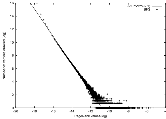
Fig.6 PageRank distribution
