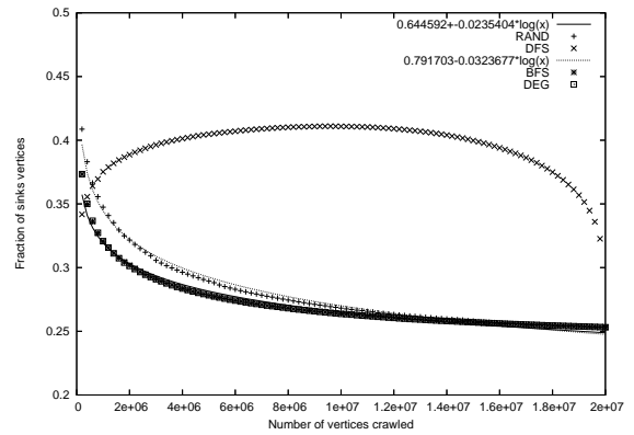
Fig.9 Evolution of the proportion of sinks (pages with no crawled successors) among crawled pages
