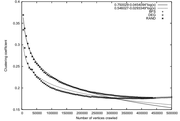
Fig.4 Evolution of clustering coefficient across time
