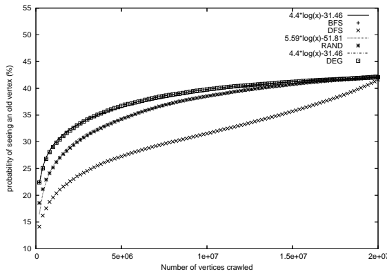
Fig.8 Evolution of the discovery rate.
