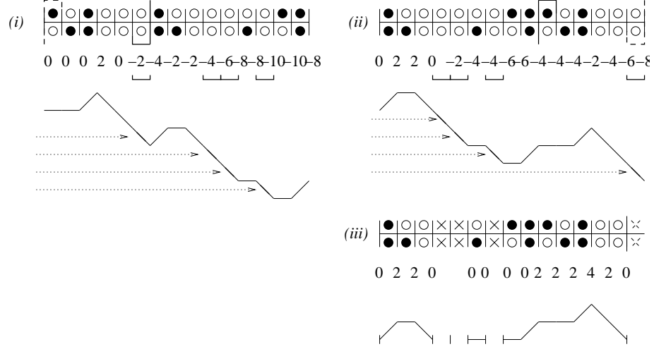
FIGURE 18. (i) An element of \bar{\Delta}_{k,m}^{\ell+1} (with \ell = 3 and column j = 6 colored), (ii) its conjugate (with column n + 1 - j colored), and (iii) the corresponding element of \bar{\Omega}_{k,m}^{\ell} . The sequence (B(j) - W(j))_{j=0..n+1} is given under each configuration and graphically represented.
