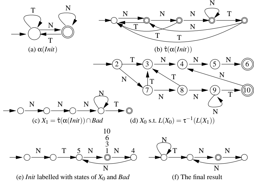
Fig. 3. An example using abstraction based on predicate languages
