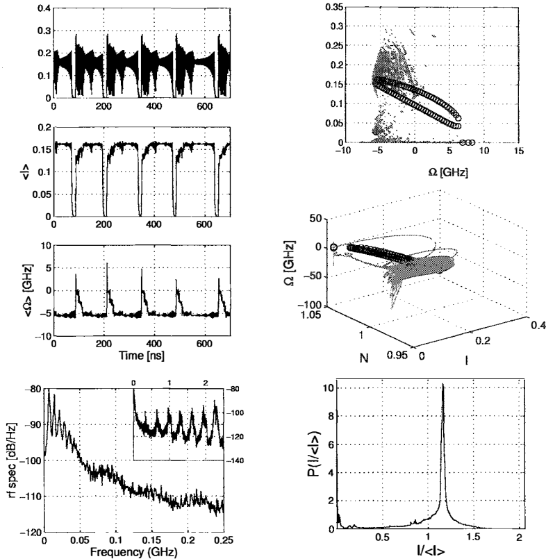
Figure 6. LFF characteristics for 2\Delta = 0.2 \text{ nm} ( 27 \text{ GHz} ), R_B(\omega_B) = 0.01 .
