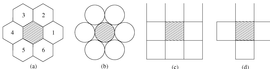
Fig. 3. Two dimensional space discretizations: hexagonal neighboring (a) is the better approximation of circles neighboring (b) while square grids allows either the 8-neighbors model (c) or the 4-neighbors model (d).
