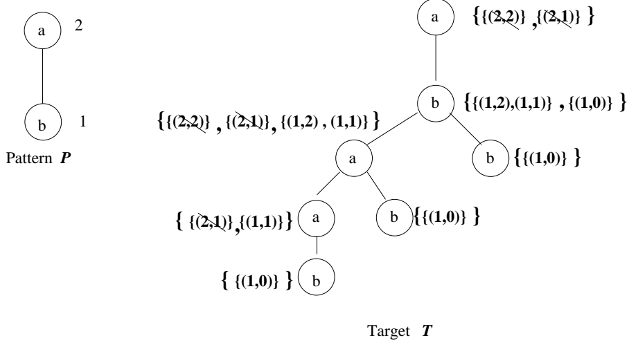
FIGURE 6. Pattern P has 5 occurrences (which are crossed with a backslash) in a 2-window (window of height at most 2) of target T .
