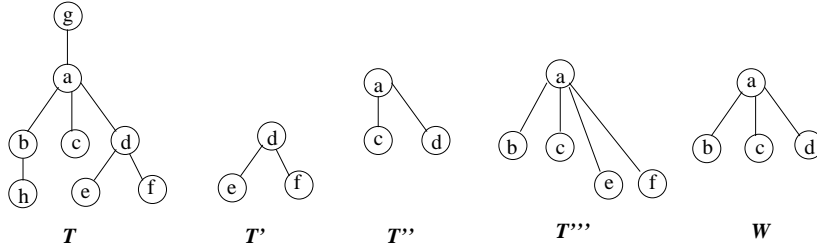
FIGURE 1. A tree T with bottom-up subtree T' , subtree T'' , embedded subtree T''' , and 1-window W .
