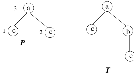
FIGURE 5. Pattern P has 2 occurrences in a window of height 2 of T .
