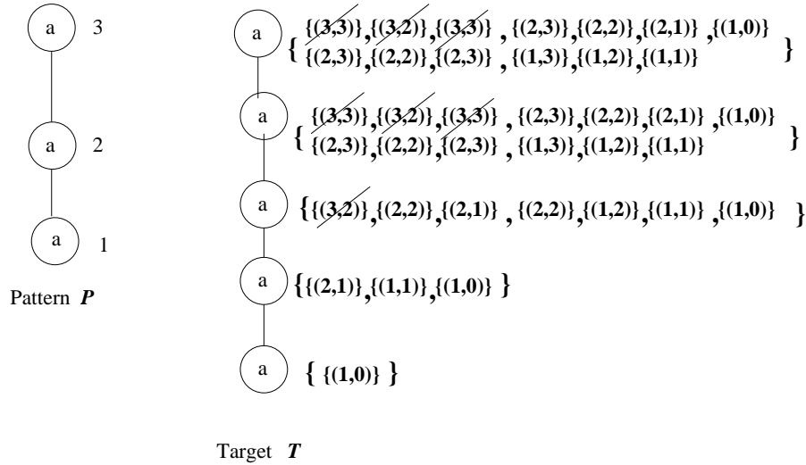
FIGURE 7. Pattern P has 7 occurrences (crossed with a backslash) in a 3-window of target T .
