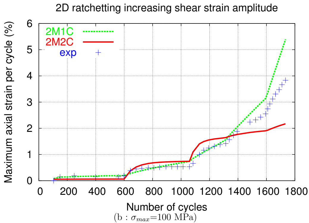
Fig. 7. Validation of the 2M1C- \beta -Model: Tension-torsion ratchetting tests with increasing the shear strain amplitude.
