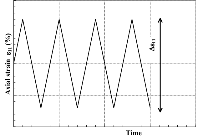
Cyclic loadings
