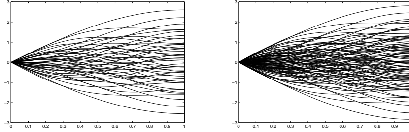
Fig. 4. Optimized functional quantization of the Brownian motion W . The N -quantizers \Gamma^N . Left: N = 48 ( d(N) = 3 ). Right: N = 96 , d(96) = 4 .
