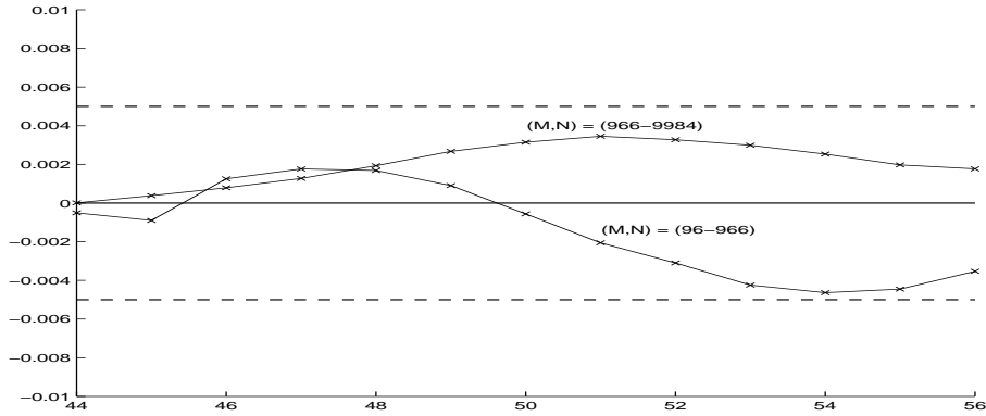
Fig. 13. Quantized diffusions based on optimal product quantization: Pricing by K -linear interpolation of Romberg log-extrapolations as a function of K (absolute error) with (M, N) = (96, 966) , (966, 9984) . T = 1 , s_0 = 50 , k = 2 , a = 0.01 , \rho = 0.5 , \vartheta = 0.1 . K \in \{44, \dots, 56\} .
