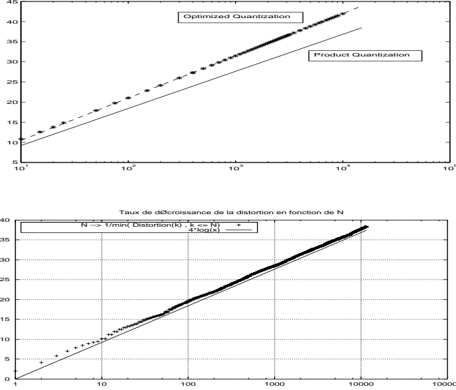
Fig. 9. Numerical quantization rates. Top (Optimal quantization). Line + + +: \log N \mapsto (\|W - \widehat{W}^N\|_2)^{-2} . Dashed line: \log N \mapsto \log N / 0.2194 . Solid line: \log N \mapsto \log N / 0.25 . Bottom (Product quantization). Line + + +: \log N \mapsto (\min_{1 \leq k \leq N} \|W - \widehat{W}^{k,prod}\|_2^2)^{-1} . Solid line: \log N \mapsto \log N / 0.25 .
