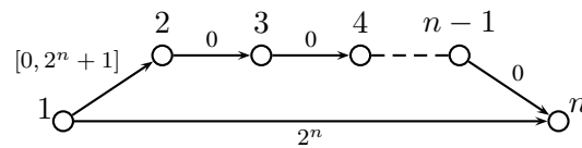
Figure 5: A critical instance of INTERVAL MIN-MAX REGRET SHORTEST PATH where the optimal min-max solution is very bad
