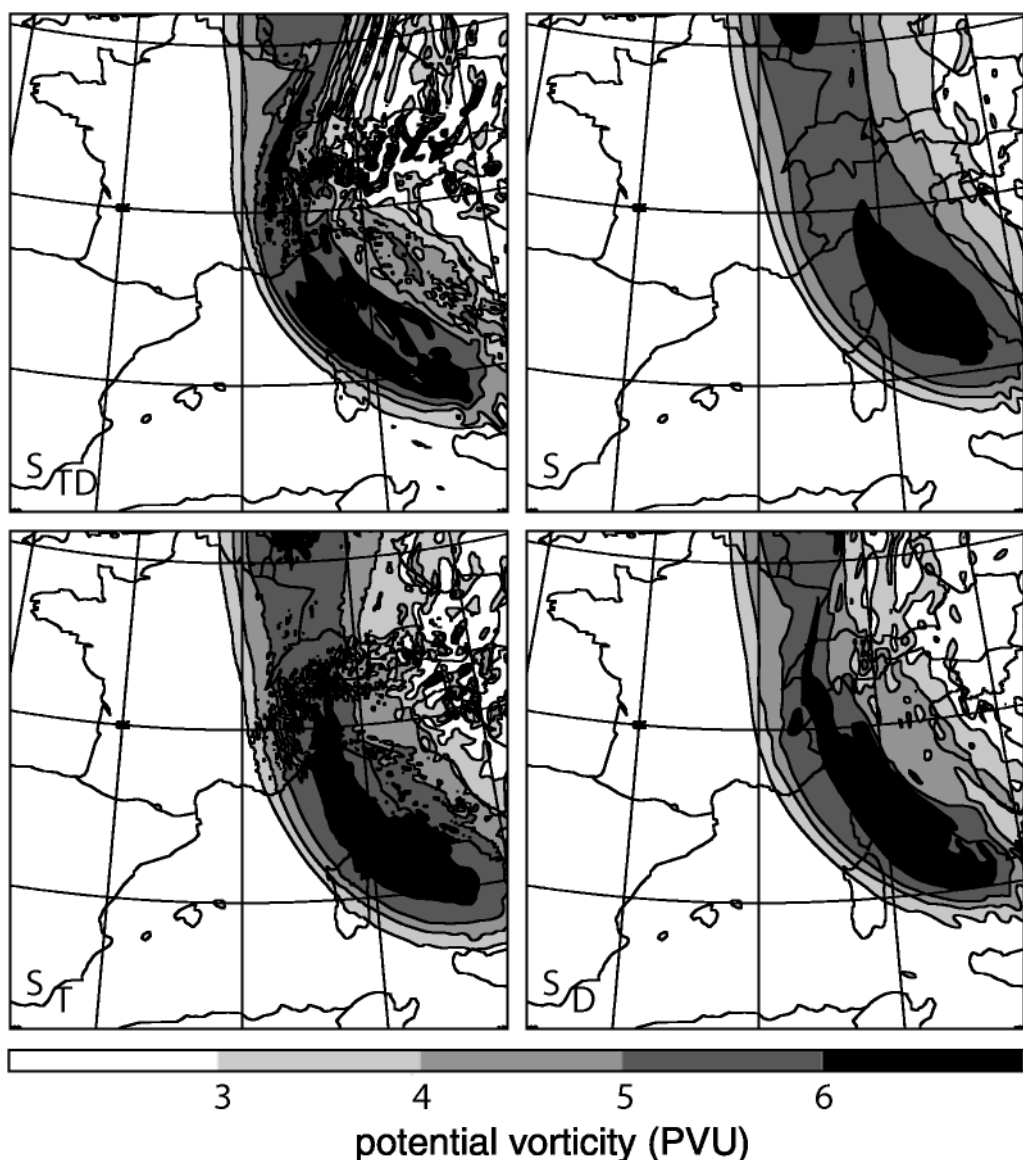
Figure 13. Vertically integrated (500–150 hPa) potential vorticity at 00 UTC 7 November 1999, for the numerical experiments S, S_T , S_D and S_{TD} (see Table 1).
