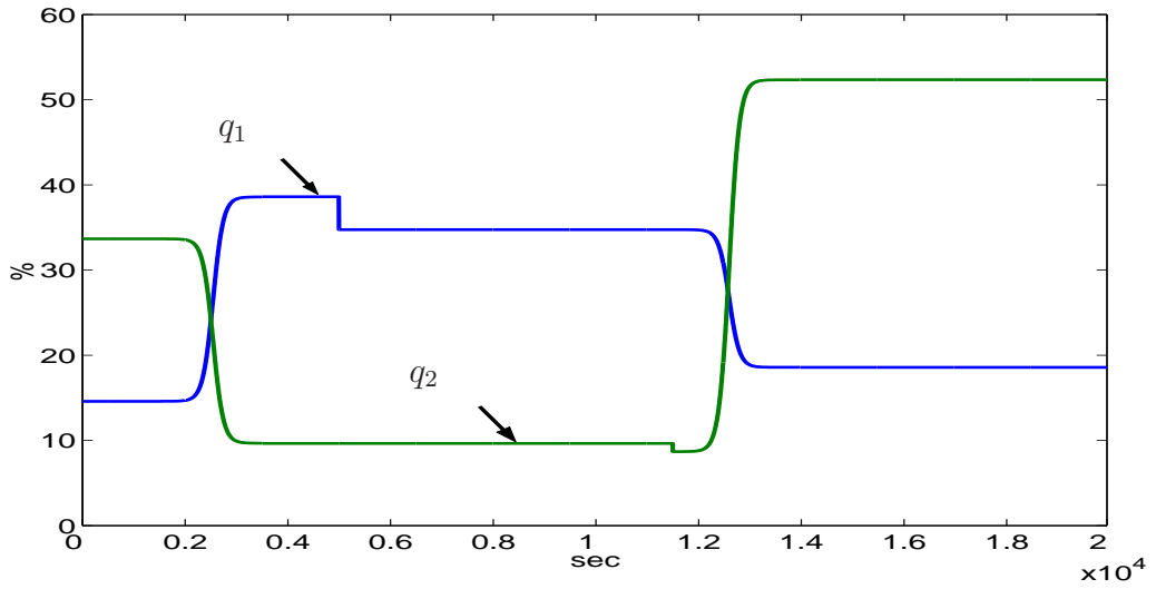
Fig. 9. Inputs in faulty case
