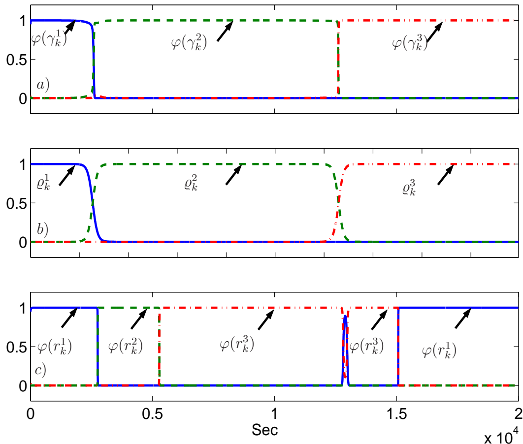
Fig. 10. Probabilities in faulty case
