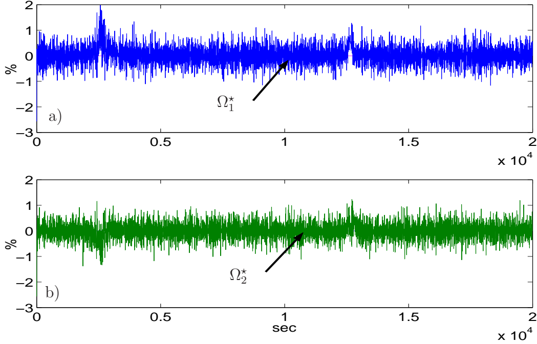
Fig. 7. Sensitive residual from the decoupling filter in fault-free case
