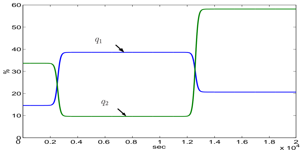
Fig. 5. Inputs in fault-free case
