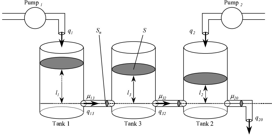
Fig. 2. Hydraulic plant
