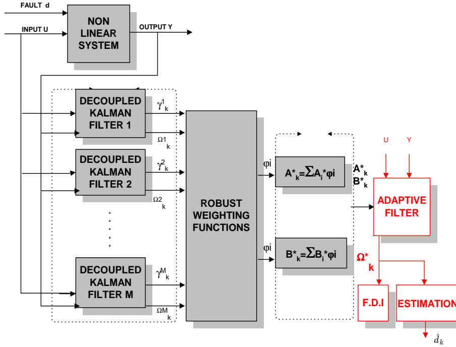
Fig. 1. General FDI scheme
