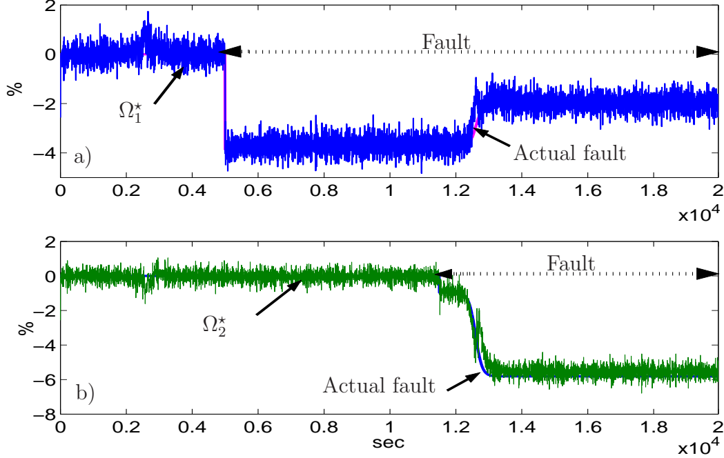
Fig. 11. Sensitive residual from the decoupling filter in faulty case
