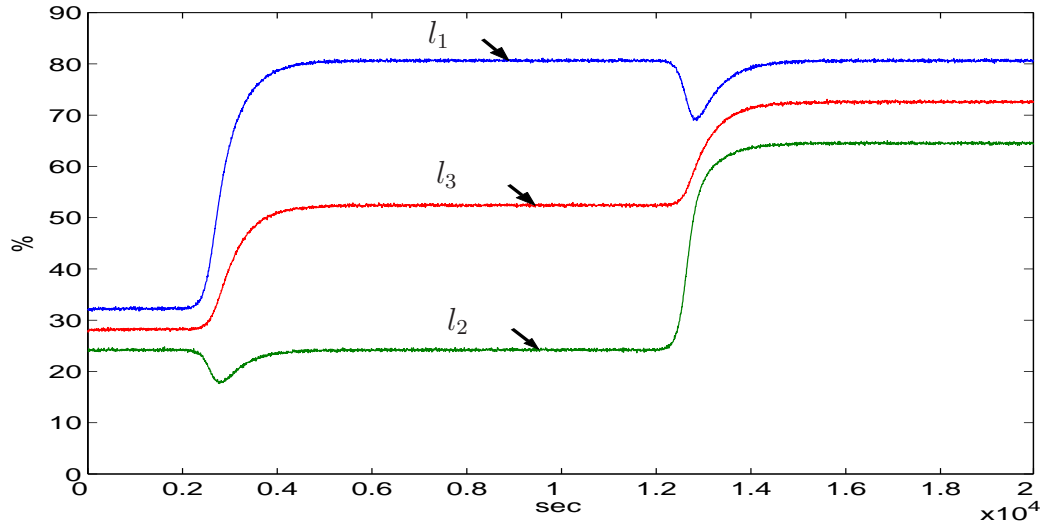
Fig. 4. Outputs in fault-free case
