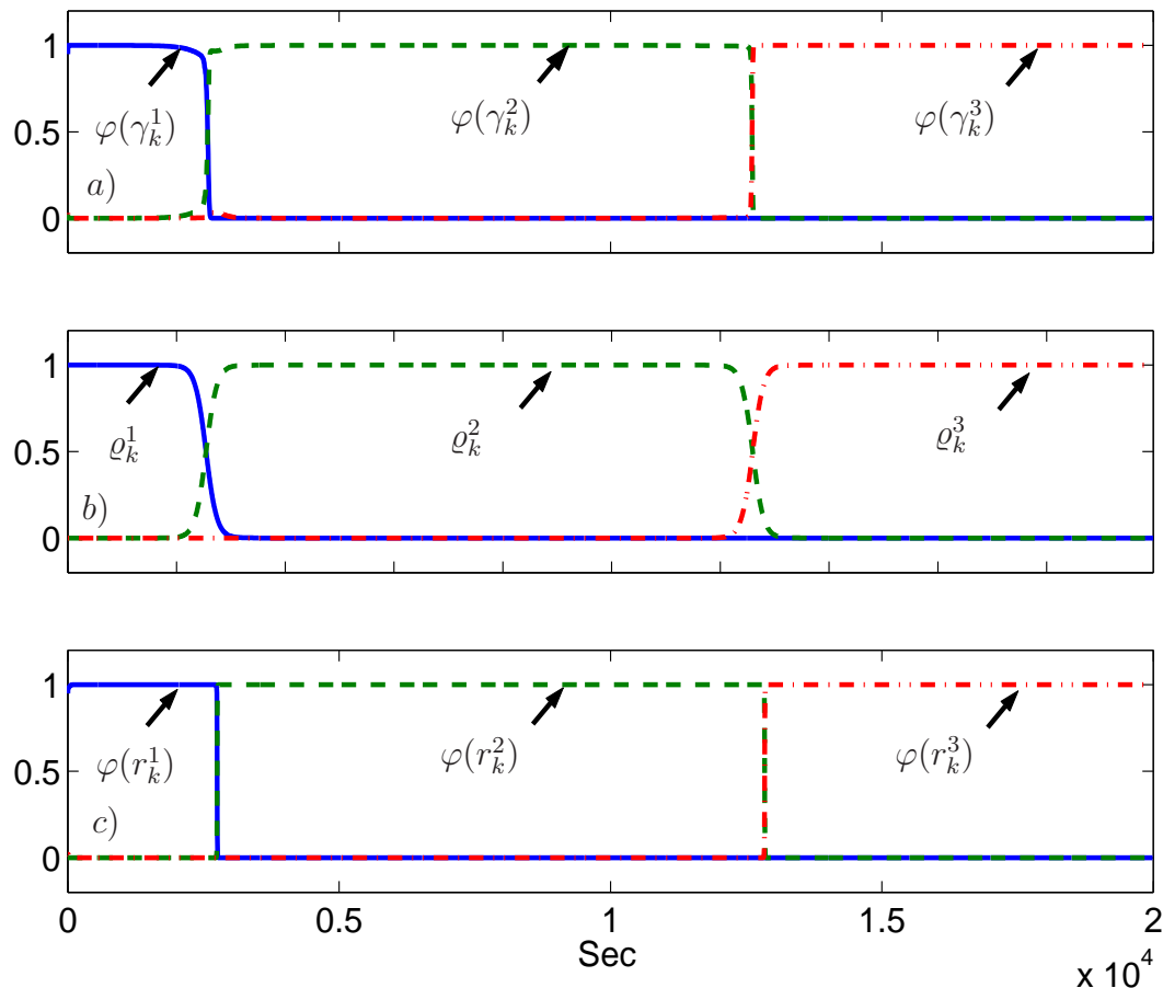
Fig. 6. Probabilities in fault-free case: a) Decoupled Kalman filter b) Actual c) Classical Kalman filter
