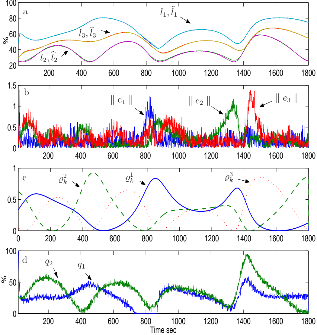
Fig. 3. System modeling: a) outputs l_v and estimated outputs \hat{l}_v b) euclidean norms \|e_v\| c) scheduling functions, d) inputs
