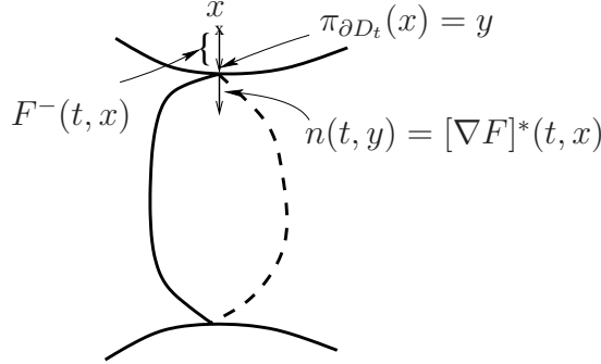
Figure 3. Orthogonal projection \pi_{\partial D_t}(x) of x \notin D_t onto the boundary \partial D_t and the related signed distance F(t, x) . Here F(t, x) < 0 and \mathbf{d}(x, \partial D_t) = |F(t, x)| = F^-(t, x) .
