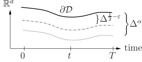
Figure 4. The two localization neighborhoods with \alpha < \frac{1}{2} - \varepsilon .
