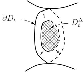
Figure 2. The boundary \partial D_t and the smaller domain D_t^\Delta .
