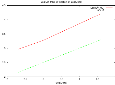
Figure 5. Error for the Monte Carlo method (without correction) as a function of \Delta , in logarithmic scales. Evaluation at x_0 = (-.7, .3, .7) .
