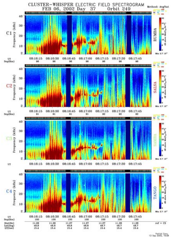
Fig. 5. Whisper spectrograms for C1, C2, C3, C4 close to the last magnetopause crossing ( \sim 08:17:20 ). The electrostatic structure is observed beginning at 08:16:15
