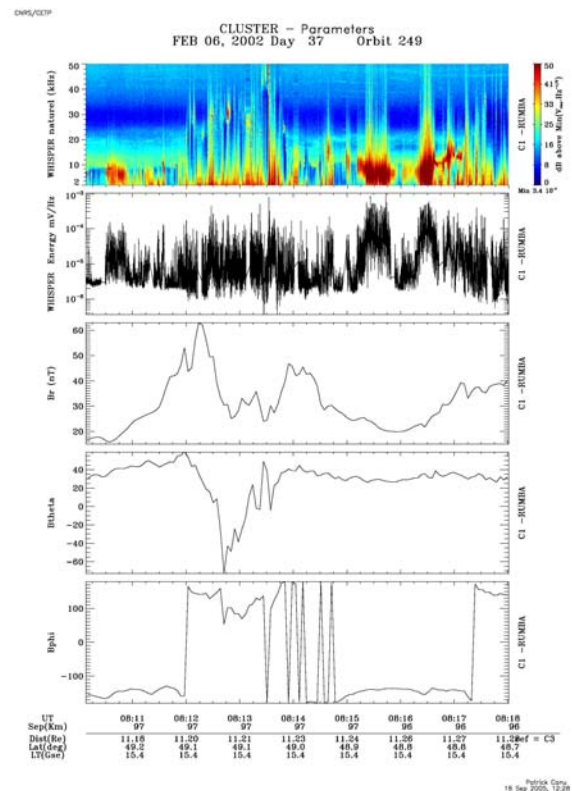
Fig. 3. Multiple crossings of the magnetopause. From top to bottom, Whisper spectrogram and integrated power (2-80 kHz) and B_r , B_\theta , B_\phi in GSE
