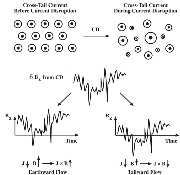
Fig. 6. Schematic of how small-scale fluctuations from localized current disruptions might lead to organized earthward or tailward flow. After Lui (2001).
