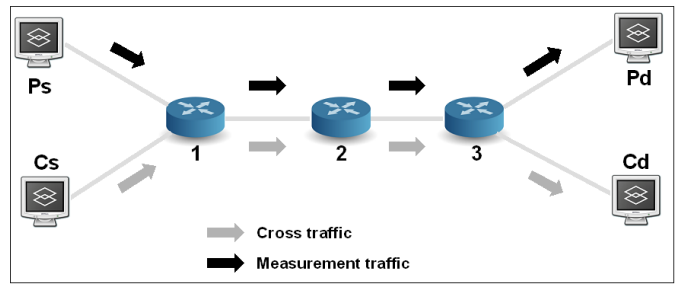
Fig. 2. Available Bandwidth Measurement Testbed.
