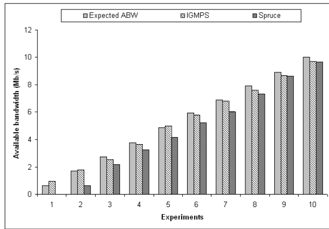
Fig. 15. Comparison of IGMPs and Spruce performance in 10 Mb/s path.
