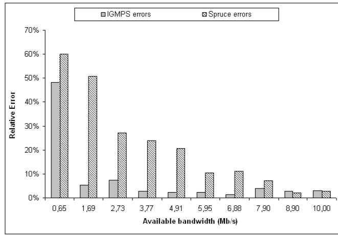
Fig. 16. Comparison of IGMPs and Spruce relative errors in 10 Mb/s path.
