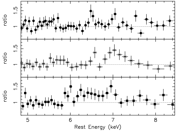
Fig. 10. The PN data/model sub-spectra of ESO 113-G010 (quasar frame) for the three time intervals. The data have been fitted assuming a power-law underlying continuum. Upper panel: 0–40 ks sub-spectrum (segment 1). Middle panel: 40–70 ks sub-spectrum (segment 2). Lower panel: 70–100 ks sub-spectrum (segment 3).
