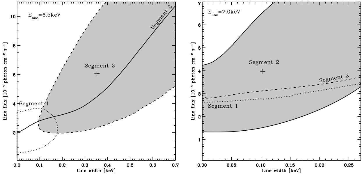
Fig. 11. Width and normalisation line contour plots at 90% confidence level ( \Delta\chi^2=4.61 ) for segment 1 (dotted-line), segment 2 (continuous line), and segment 3 (dashed-line). Left panel: line at 6.5 keV. For segment 2, only an upper limit is found, corresponding to the continuous line. Right panel: line at 7.0 keV. For segments 1 and 3, only an upper limit is found.
