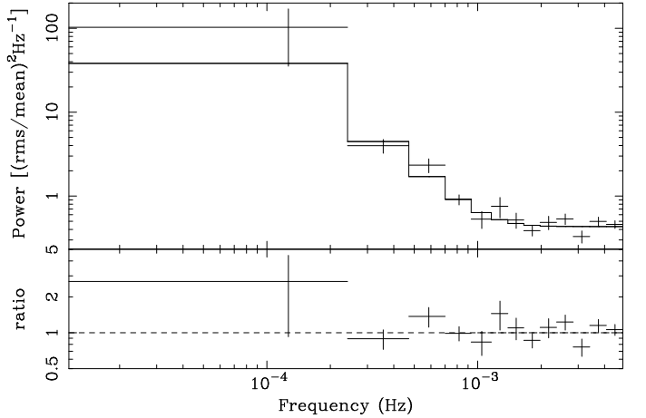
Fig. 3. 0.3–10 keV PSD of ESO 113-G010, including the ratio of the data to an exponentially cut-off power-law (with low-frequency slope \alpha = -1 ), plus constant Poisson noise component (model shown as solid line).
