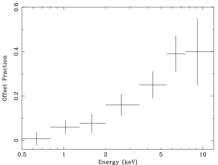
Fig. 6. Fractional offset spectrum, showing fractional constant offsets (y-axis intercept divided by mean flux) for a linear plus constant model fitted to various energy bands versus the 0.3–0.5 keV reference band. In the case that the two-component model for spectral variability is correct, the offset spectrum shows lower limits on the strength of the constant component relative to the mean spectrum.
