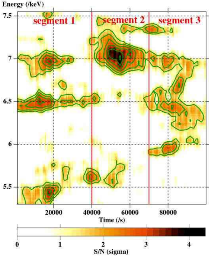
Fig. 9. Energy-time map. The energy values are in the quasar frame. The contours represent 1.5–4.0 sigma above the continuum (in 0.5 increments), with darker bins representing an excess above the continuum. The segments 1-3 (delimited by red vertical lines) correspond to the time selections used for the time-resolved spectroscopic analysis. See text for explanation.
