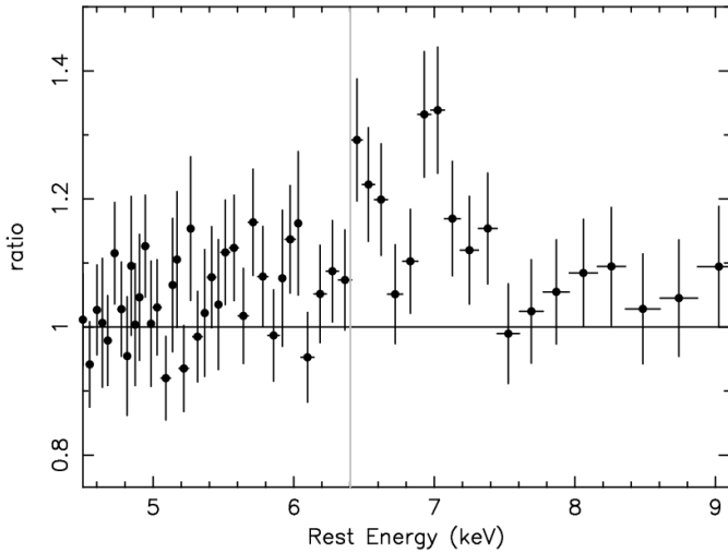
Fig. 8. Fe K line profile (quasar frame) when PN time-averaged data are fit with a power-law continuum. For presentation, the data have been re-binned into groups of 10 bins for PN, after group of a minimum of 100 counts per bin were used for the fit. The grey vertical line corresponds to 6.4 keV.
