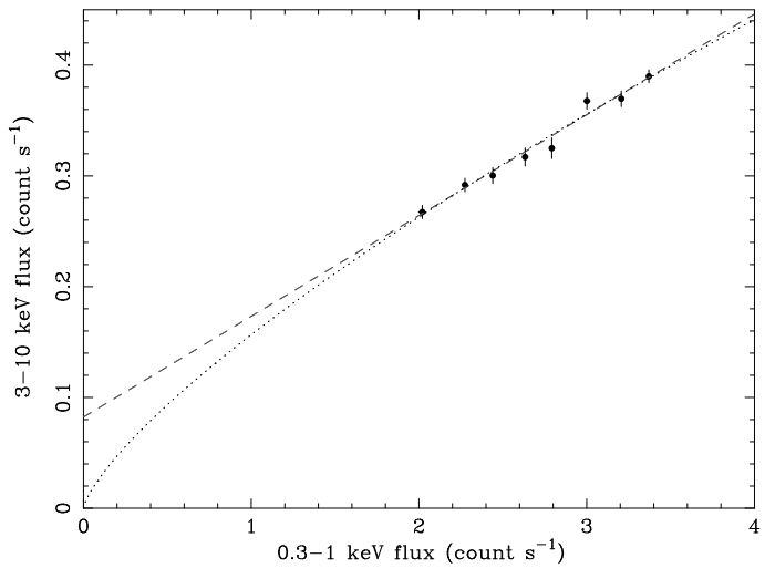
Fig. 5. 3–10 keV versus 0.3–1 keV binned flux-flux plot of ESO 113-G010, compared with a best-fitting linear plus constant model (dashed line, representing two-component spectral variation) and a simple power-law (dotted line, representing high energy spectral pivoting). The two models are indistinguishable over the relatively narrow flux range covered by the data.
