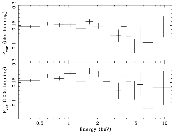
Fig. 4. The rms-spectra of ESO 113-G010, for light curve bin times of 5 ks (top) and 500 s (bottom). See text for details.
