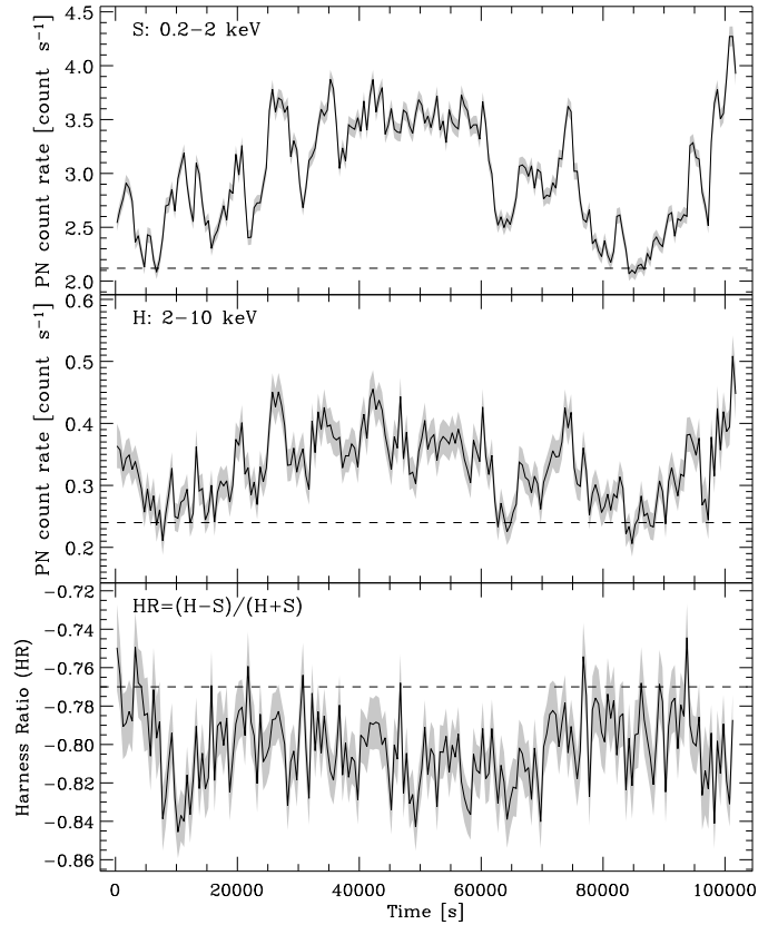
Fig. 1. Soft (S: 0.2–2 keV) and hard (H: 2–10 keV) 500-s resolution (background-subtracted) PN light curves of ESO 113-G010 (upper and middle panels, respectively), together with the hardness ratio between the two bands (lower panel). The grey stripes correspond to the 1\sigma error bars. For comparison the count rate and hardness ratio level found during the 4 ks May 2001 observation are reported (dashed lines).
