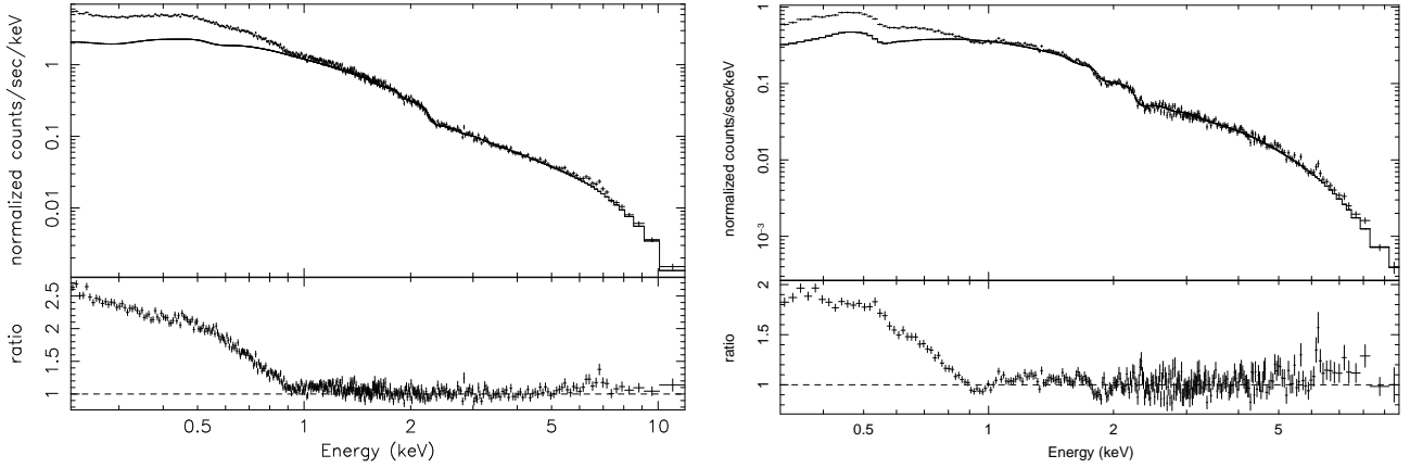
Fig. 7. Spectra of ESO113-G010 (in the observer frame) observed in November 2005. A power-law has been fitted to the 2–5 keV data and extrapolated to lower and higher energies. A significant soft X-ray positive residual is seen below 1 keV, as well as the presence of a Fe K\alpha complex near 6–7 keV. For presentation, the data have been re-binned into groups of 15 bins for PN (10 for MOS), after group of a minimum of 100 and 50 counts per bin were used for the fit for the PN and MOS respectively. Left panel: 0.2–12 keV PN spectrum. Right panel: co-added MOS 0.3–10 keV spectrum.
