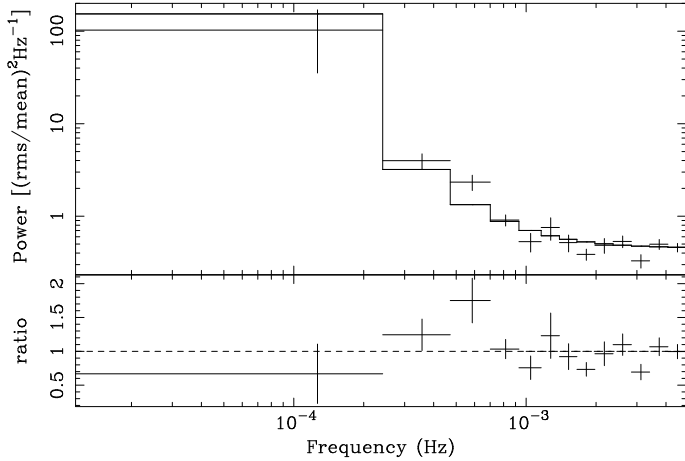
Fig. 2. 0.3–10 keV PSD of ESO 113-G010, including the ratio of the data to the best-fitting power-law plus constant noise component model (model shown as solid line).
