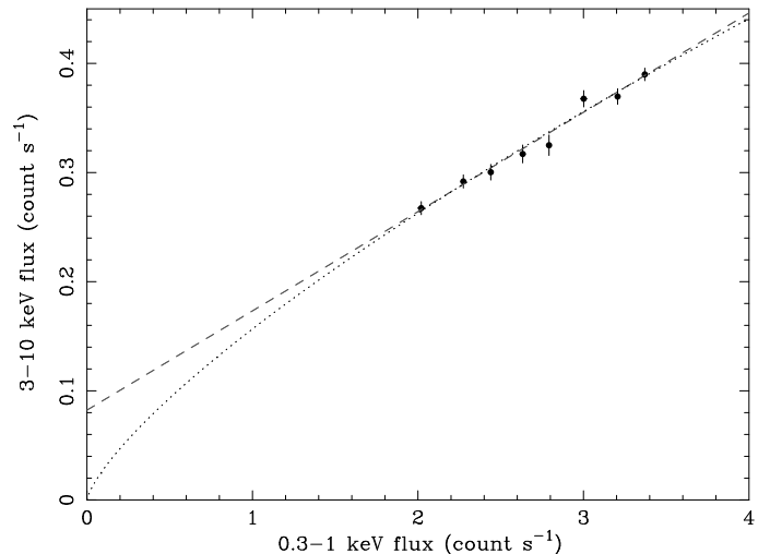
Fig. 5. 3–10 keV versus 0.3–1 keV binned flux-flux plot of ESO 113-G010, compared with a best-fitting linear plus constant model (dashed line, representing two-component spectral variation) and a simple power-law (dotted line, representing high energy spectral pivoting). The two models are indistinguishable over the relatively narrow flux range covered by the data.
