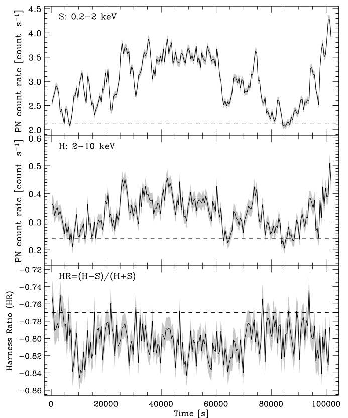
Fig. 1. Soft (S: 0.2–2 keV) and hard (H: 2–10 keV) 500-s resolution (background-subtracted) PN light curves of ESO 113-G010 (upper and middle panels, respectively), together with the hardness ratio between the two bands (lower panel). The grey stripes correspond to the 1\sigma error bars. For comparison the count rate and hardness ratio level found during the 4 ks May 2001 observation are reported (dashed lines).
