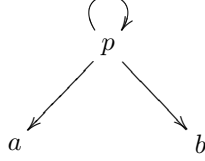
FIGURE 1. The quiver E corresponding to p = p + a + b .
