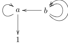
FIGURE 3. A quiver whose graph monoid retracts to \mathbb{Z}^\infty .
