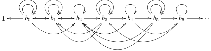
FIGURE 4. A quiver that represents \mathbb{Z}^\infty .
