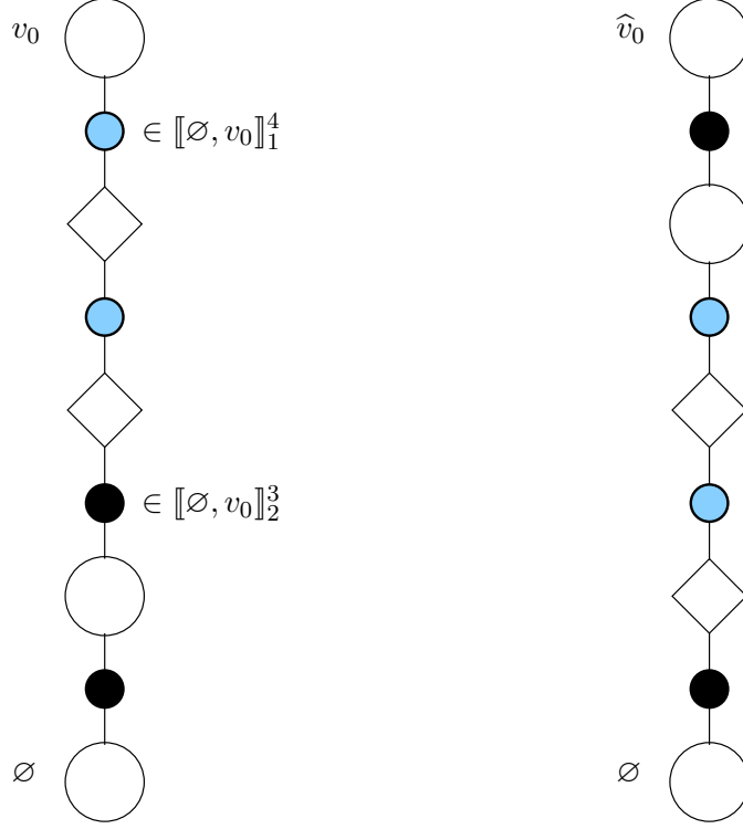
Figure 1: The branch leading from \emptyset to v_0 , and the corresponding branch in the tree \hat{\mathbf{t}}^{(v_0)} : the branch is put upside-down and the vertices of [\emptyset, v_0]_2^3 and [\emptyset, v_0]_1^4 interchange their roles.
