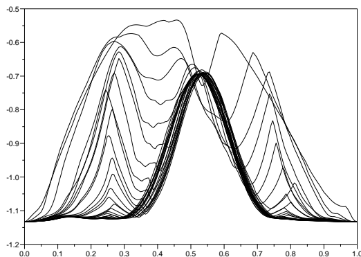
FIGURE 3. Energy along the successive deformed paths generated by Algorithm 2 for the computation of the first singlet excited state of \text{H}_2 , with R = 1 \text{ \AA} .
