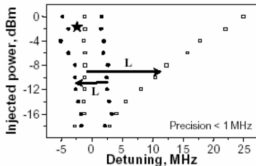
Fig. 4. Mapping of an injected fibre laser at r = 1.7 for an increasing (square) or a decreasing (circles) detuning, both for increasing injected powers.
