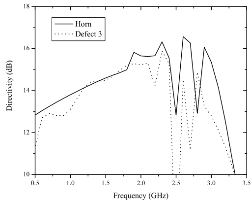
Figure 5: Directivity of the CEBG structures with different defect configurations
