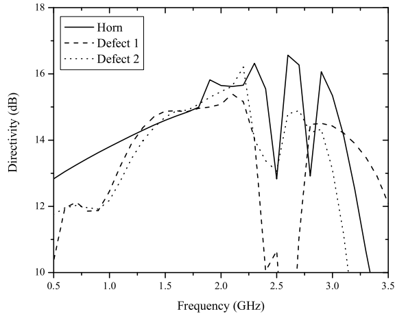
Figure 3: Directivity of the CEBG structures with different defect configurations
