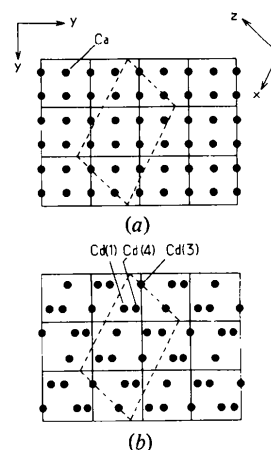
Fig. 3. Unit-cell relation between scheelite (solid lines) and \text{KCd}_4(\text{VO}_4)_3 (dotted lines): (a) projection of the Ca atoms on the (001) plane of \text{CaWO}_4 , (b) projection of the Cd(1), Cd(3) and Cd(4) atoms on the (010) plane of \text{KCd}_4(\text{VO}_4)_3 .
