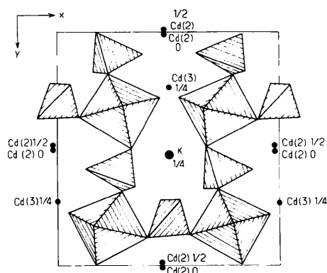
Fig. 2. Projection of a fragment of the KCd_4(VO_4)_3 structure on the (001) plane.
