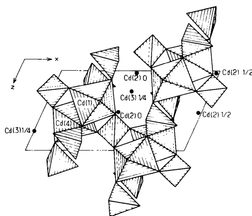
Fig. 1. Projection of a sheet of the KCd_4(VO_4)_3 structure on the (010) plane.
