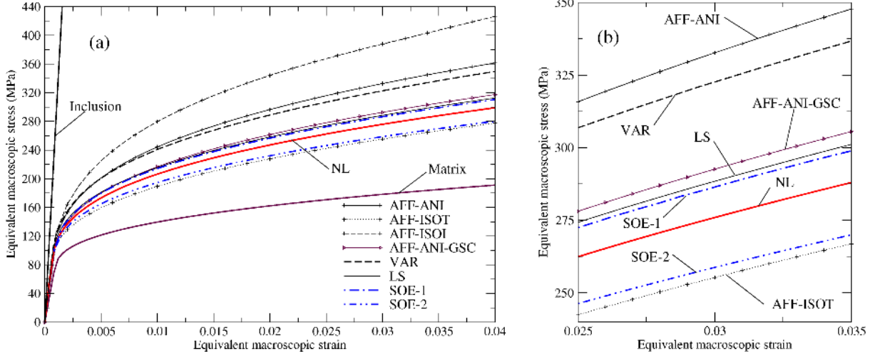
Fig. 1. Macroscopic tensile curves of a two-phase composite for different linearization procedures. Inclusion volume fraction f_p = 30\% , inclusion elastic properties: E_p = 400 GPa, \nu_p = 0.2 . Matrix elastic properties: E_m = 75 GPa, \nu_m = 0.3 ; matrix power-law properties: m = 0.3895 , \varepsilon_0 = 100\% , \sigma_0 = 416 MPa, with a threshold stress \sigma_y = 75 MPa. Full curves (a) and zoom (b).
