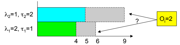
Figure 2: Illustration of the difference between HEFT (that will map task i on processor 1) and RHEFT (that will map task i on processor 2)
