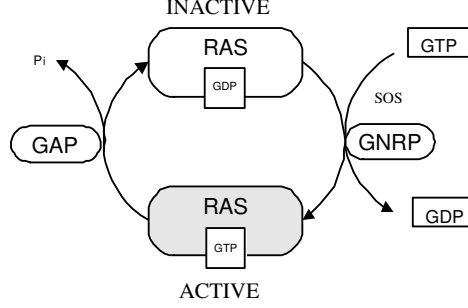
Fig.1. Ras Activation
